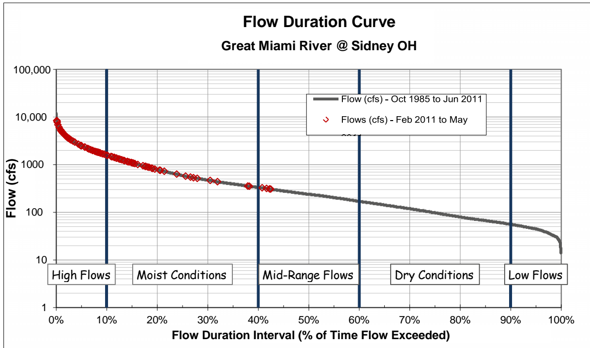
Figure E-1 Flow duration curve for data collected at USGS automatic gauge 03261500 (Great Miami River at Sidney OH) for the period October 1985 through June 2011. Flows during 2011 that occurred between February 16 and May 31 are highlighted in red. All values reported as average daily flow in cubic feet per second (cfs).
