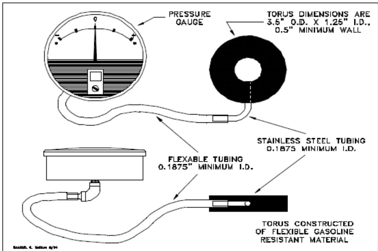
Torus Pressure Test Assembly
