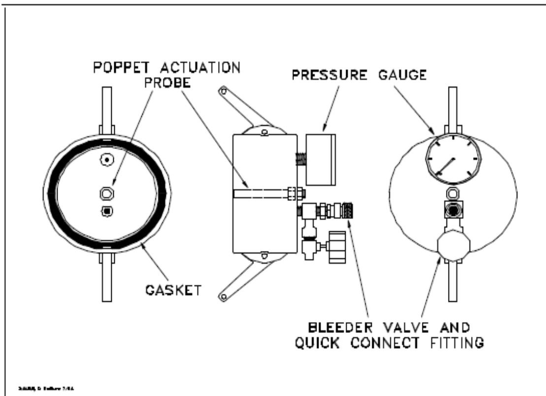
Vapor Coupler Test Assembly
