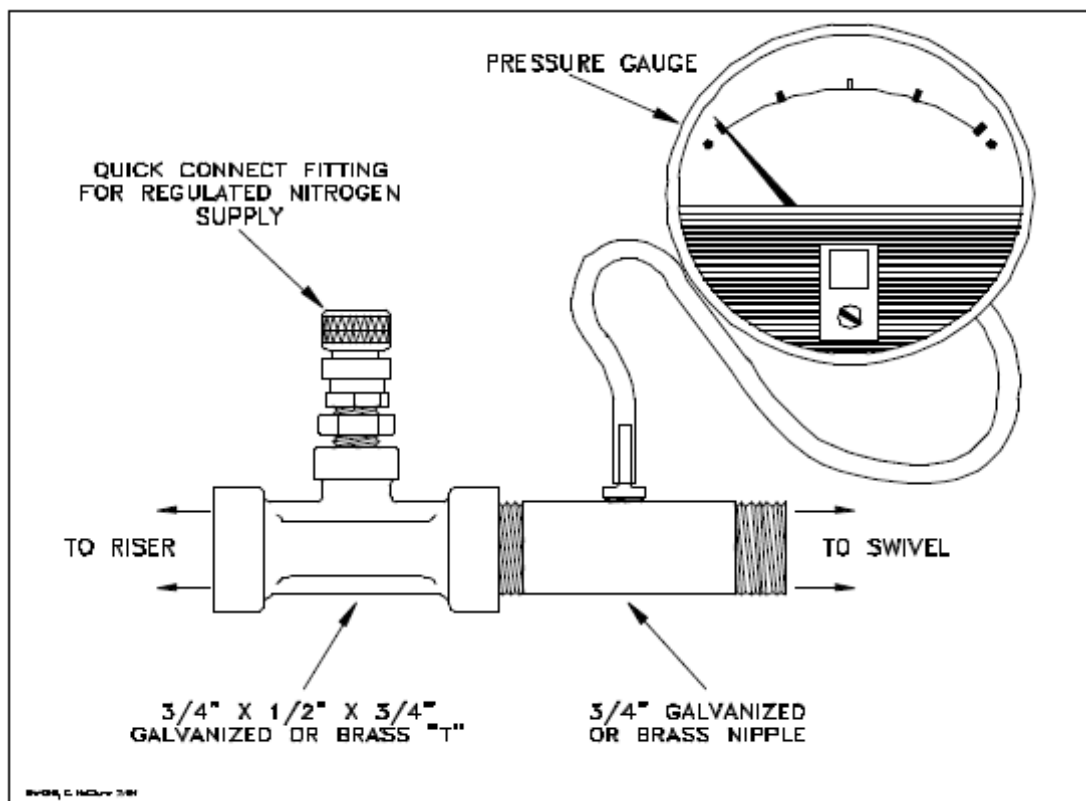
"T" Connector Assembly
