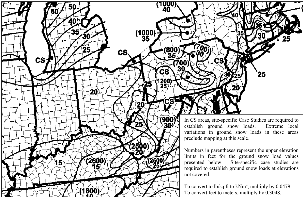
FIGURE 1608.2 GROUND SNOW LOADS, p_g , (psf)
