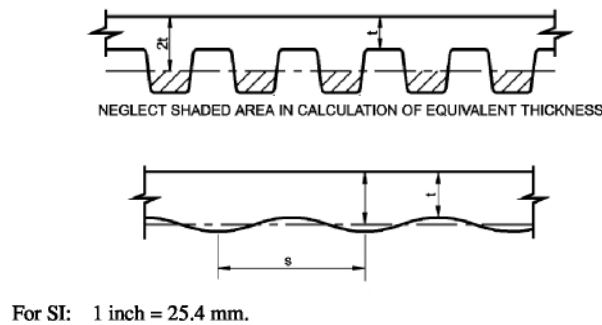
FIGURE 721.2.2.1.3 SLABS WITH RIBBED OR UNDULATING SOFFITS
