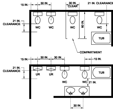
FIGURE 405.3.1 FIXTURE CLEARANCE
