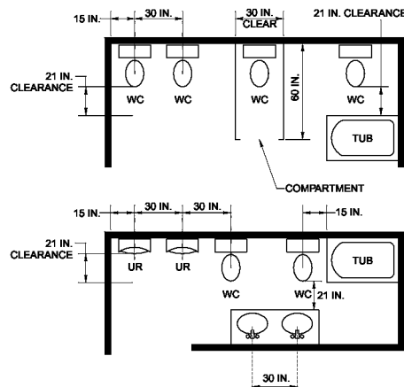
FIXTURE CLEARANCE
